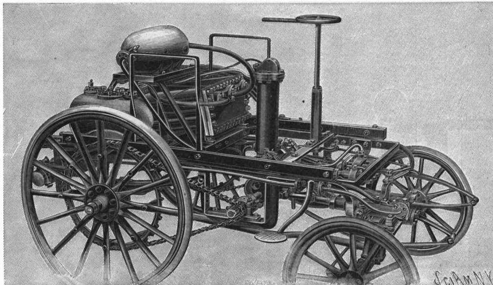
Fig. 2.—ETHER-MOTOR CARRIAGE.
