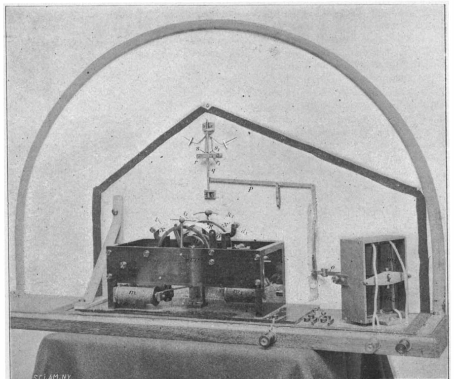
Fig. 6.—Receiving Instrument.
