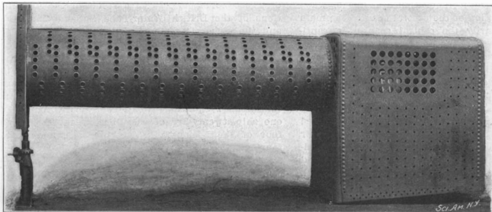
The Firebox and Water-Tube Flue.
