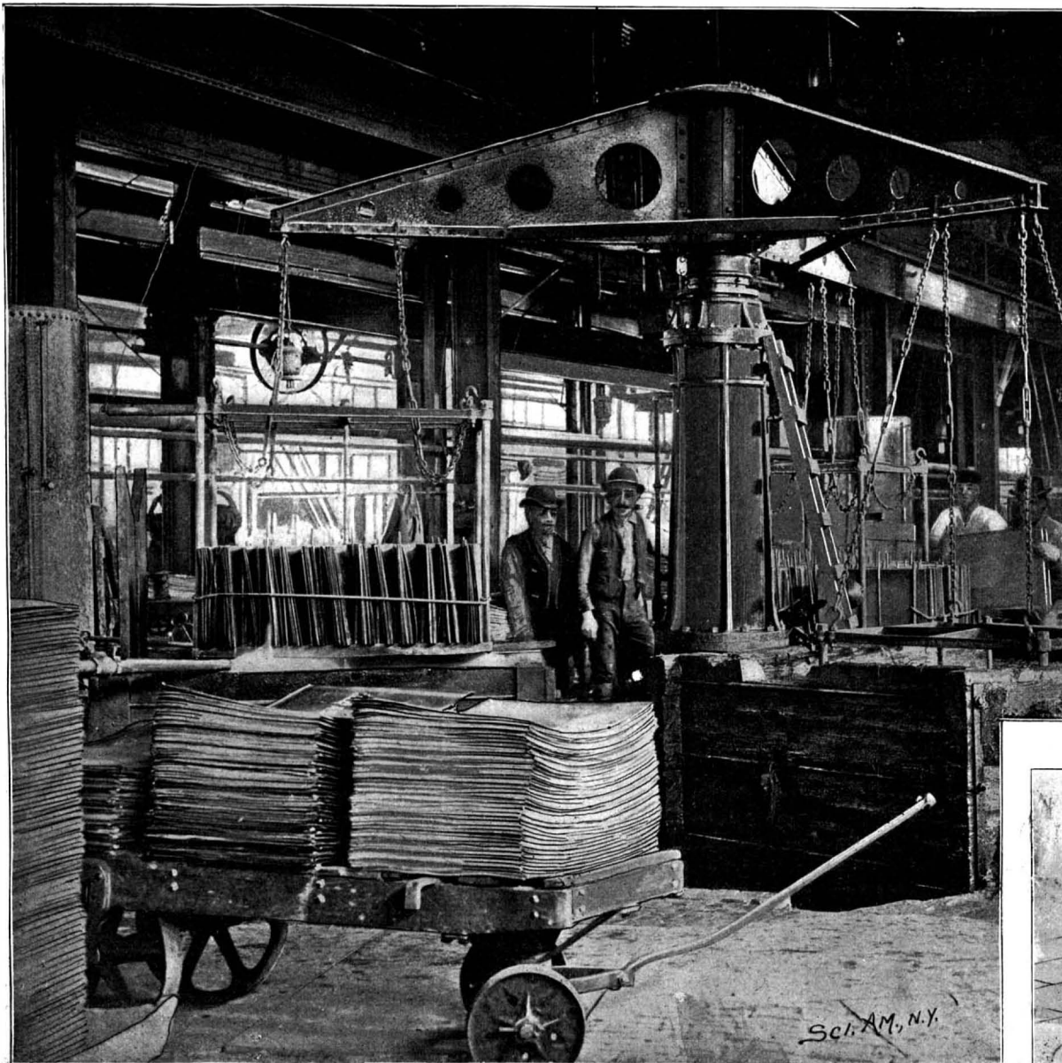
The Pickling Machines for Cleaning Plates Preparatory to Tinning.
