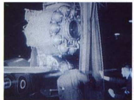
TURBOJET ENGINE is being fitted into the Gloster-Whittle E.28/39 aircraft during the spring of 1941.
