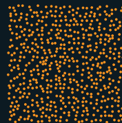
WIMPs created early in the big bang
