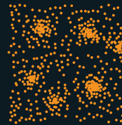
They slow down and seed galaxies
