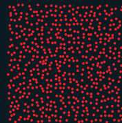
They decay to fast super-WIMPs
