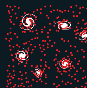
Galaxies form
