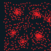
Super-WIMPs slow down and seed galaxies
