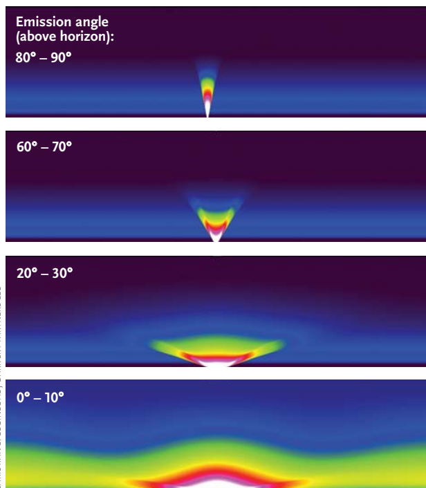
LIGHT'S LONG REACH A computer simulates the skylight visible at a mountaintop observatory 50 km away from (and 2 km above) a strong light source. Light directed straight up escapes to space with little atmospheric interaction. However, light emitted just above horizontal scatters strongly and creates the most skylight. Blue light is scattered far more strongly than red light.
